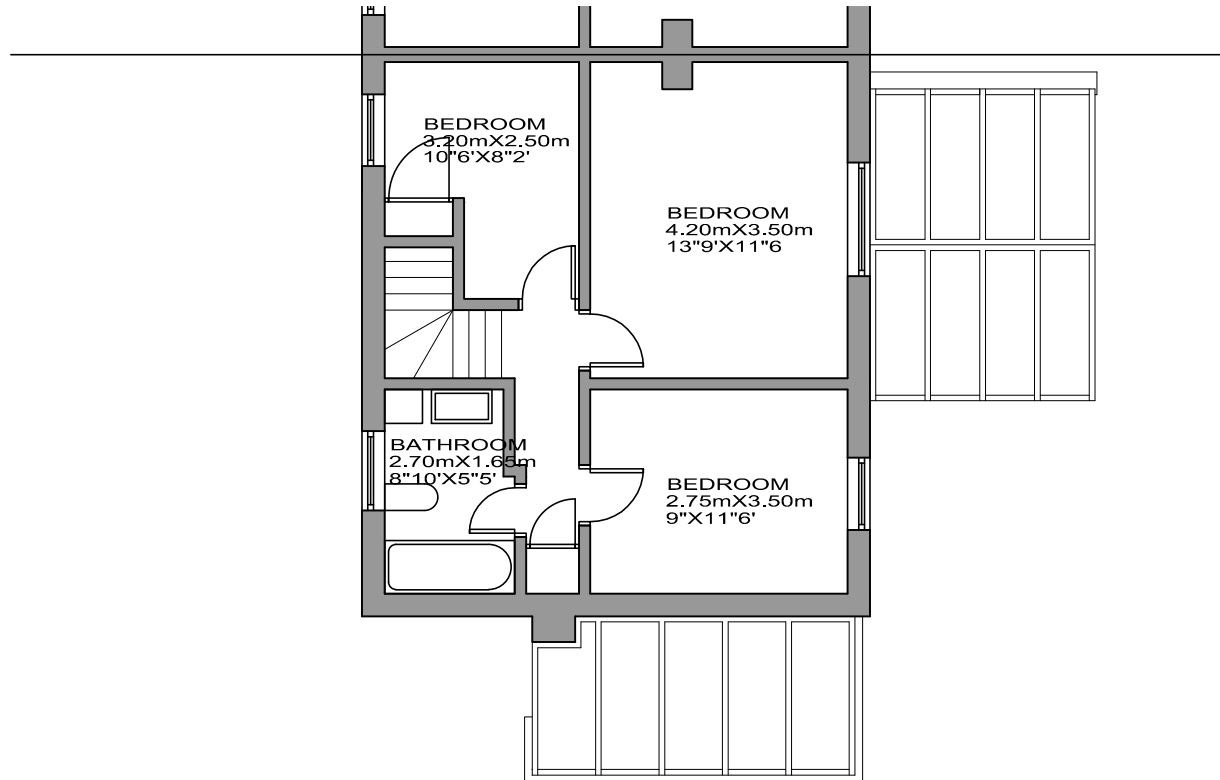
FIRST FLOOR PLAN NET AREA 41.1 SQM / 452 FT2
